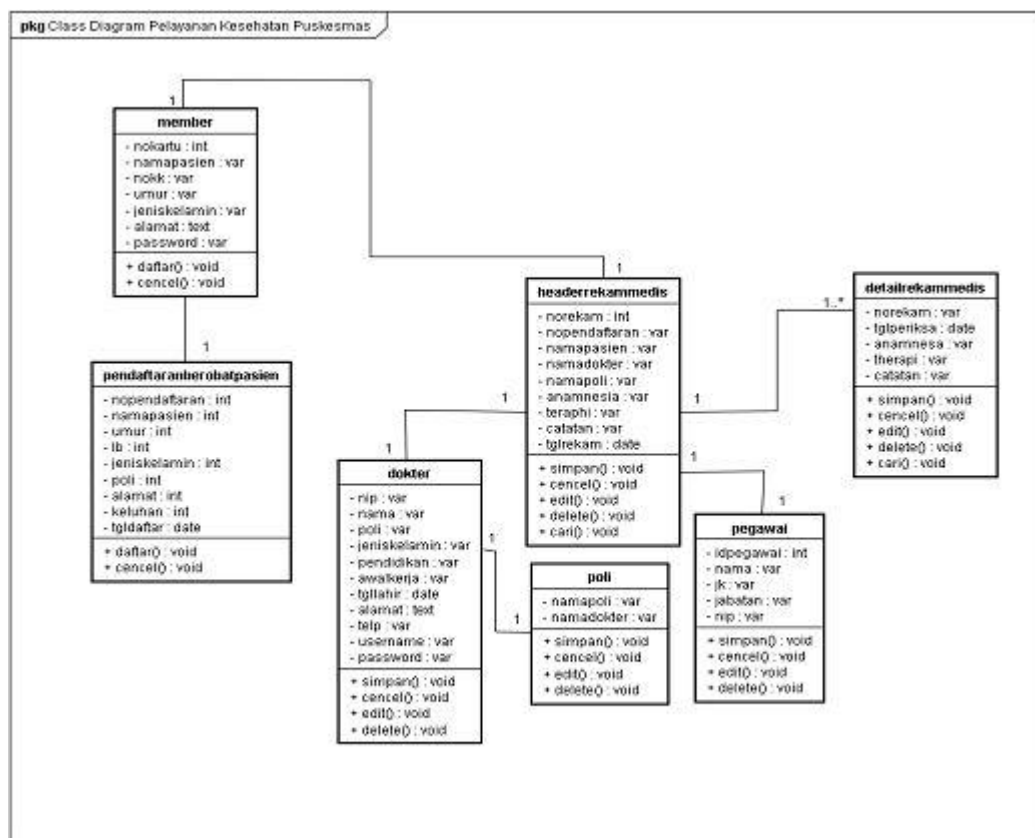
Gambar 3.8 Class Diagram
