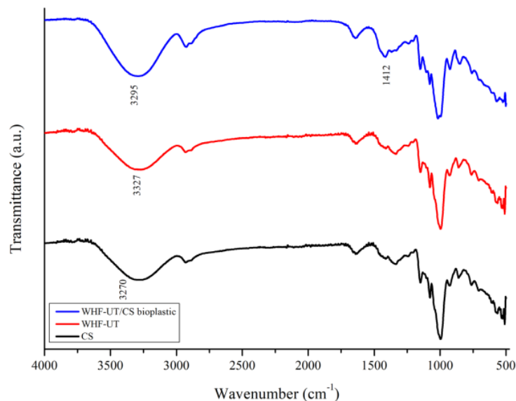
Figure 5. FT-IR spectra of WHF-UT/CS bioplastic
