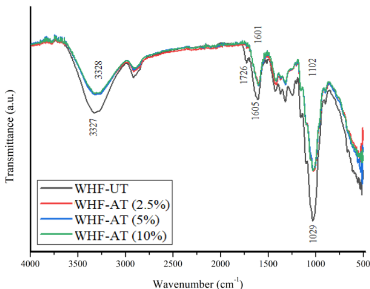
Figure 4. FT-IR spectra of WHF
