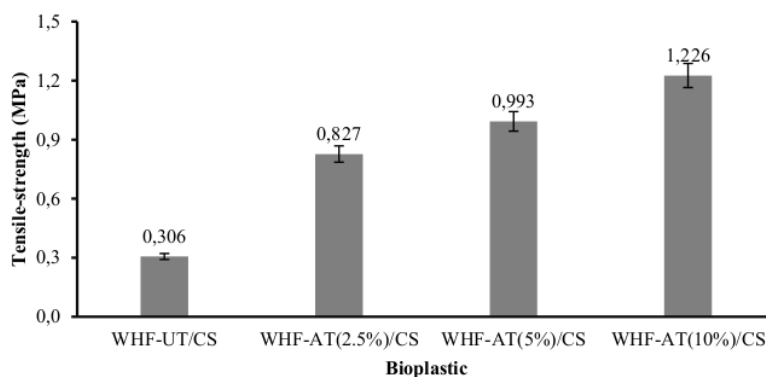
Figure 7. Tensile-strength of bioplastic film
