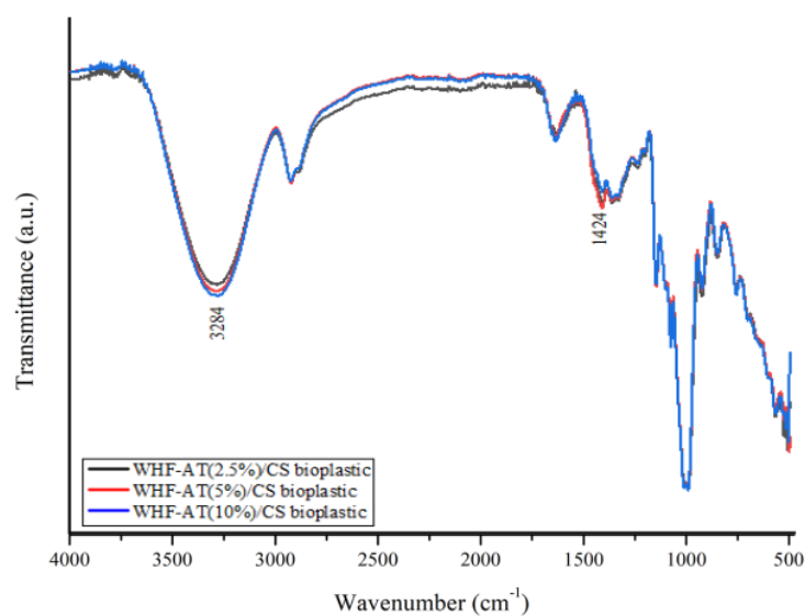
Figure 6. FT-IR spectra of WHF-AT/CS bioplastic.
