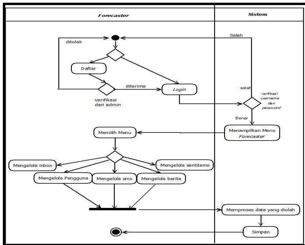
Gambar 3.7 Activity Diagram Forecaster
