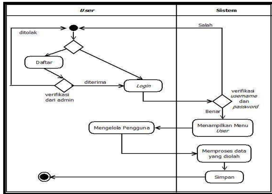
Gambar 3.8 Activity Diagram User
