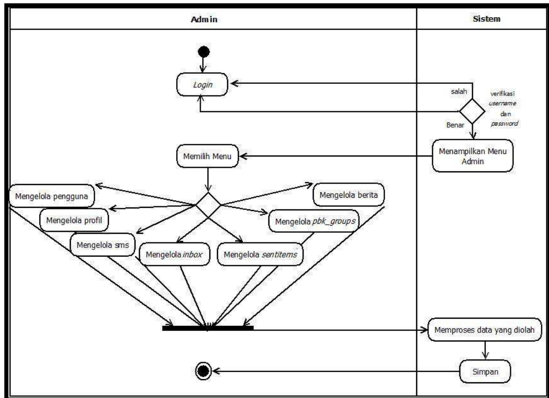
Gambar 3.6 Activity Diagram Admin
