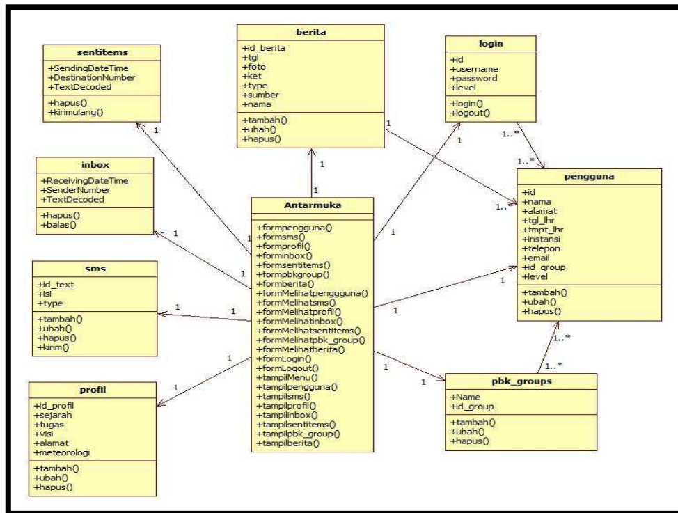
Gambar 3.5 Class Diagram SMS Gateway
