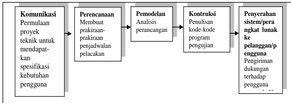
Gambar 1.1 Model Waterfall
