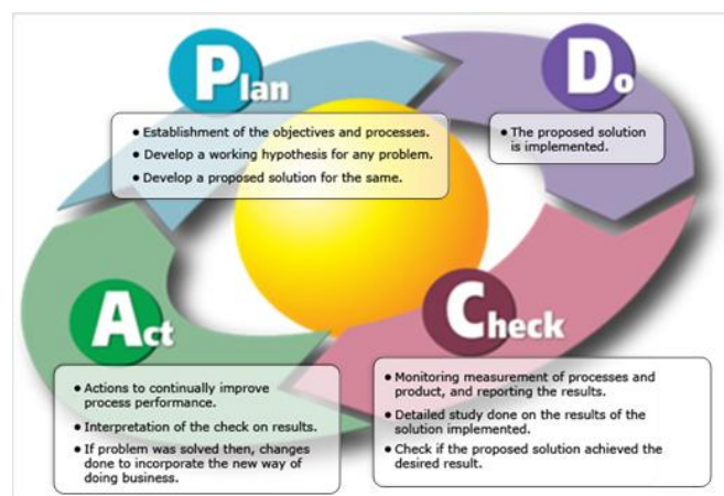
Fig.1: PDCA cycle
